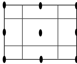
(8) pgg2
