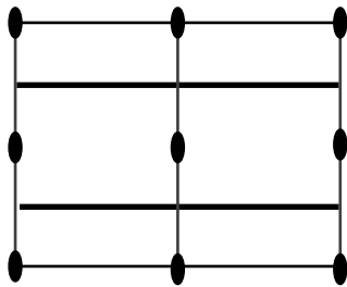
(7) pmg2
