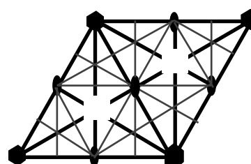
(17) p6mm
