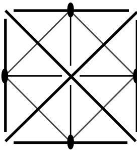
(11) p4mm
