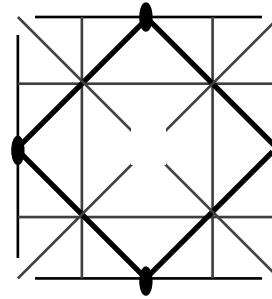
(12) p4gm
